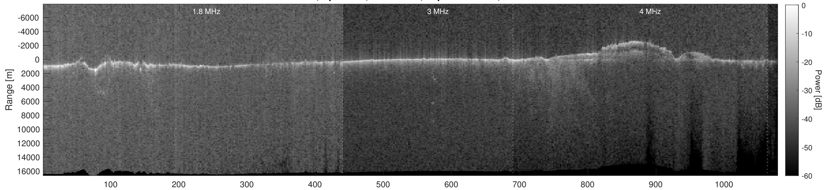
Orbit 3762, Depth-Corrected Cluttergram
