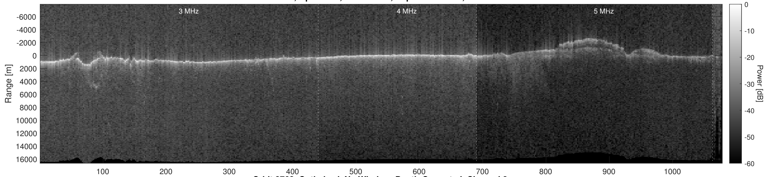
Orbit 3762, Optimized, No Window, Depth-Corrected, Channel 2
