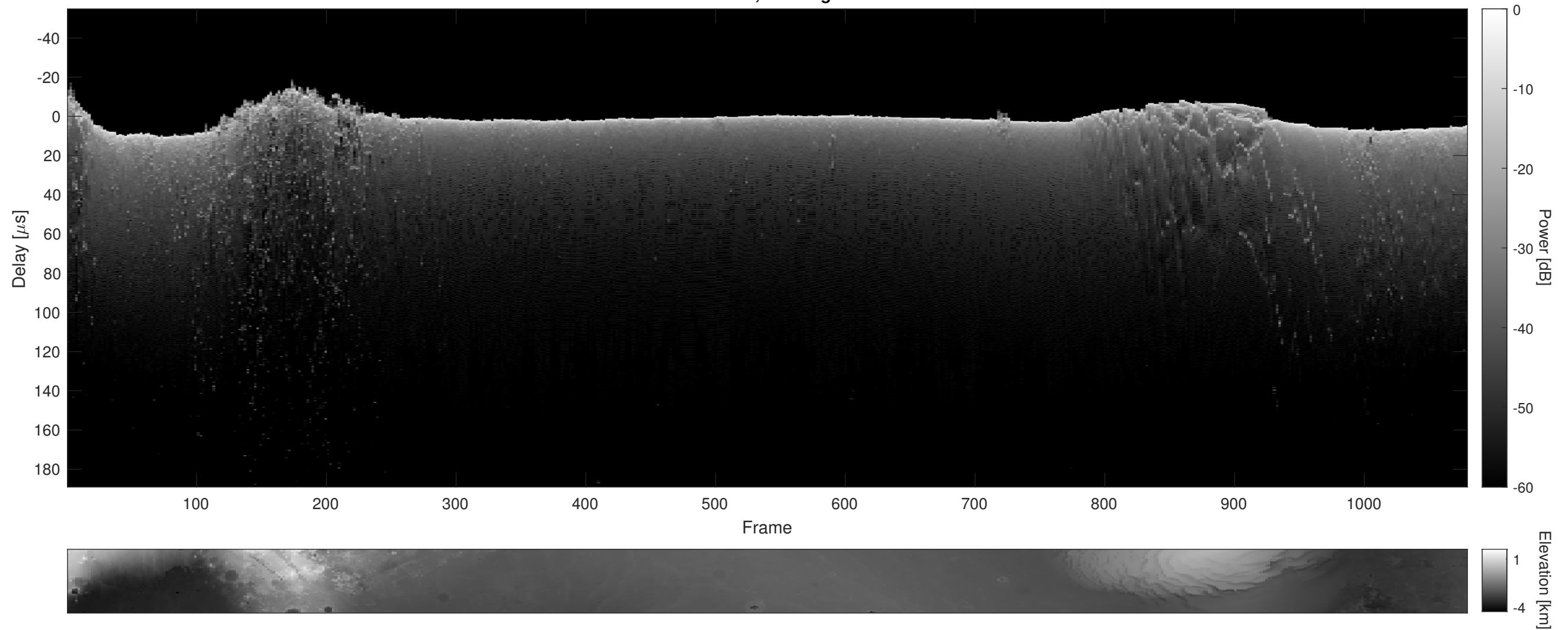
Orbit 3763, Cluttergram
