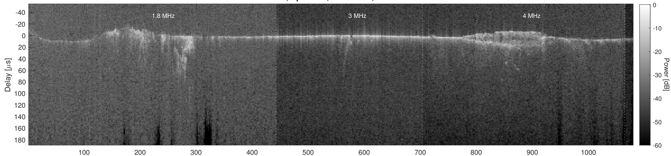
Orbit 3763, Cluttergram
