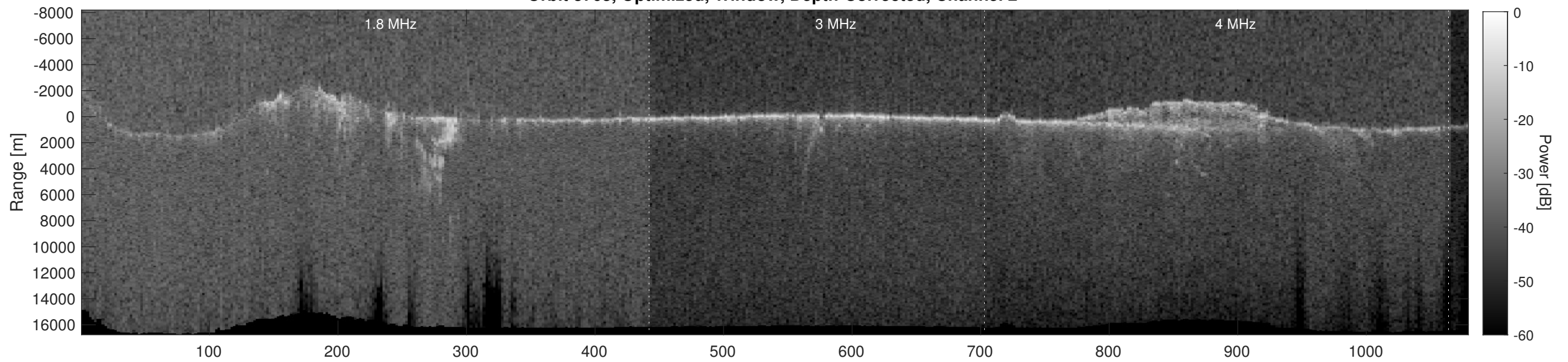
Orbit 3763, Depth-Corrected Cluttergram
