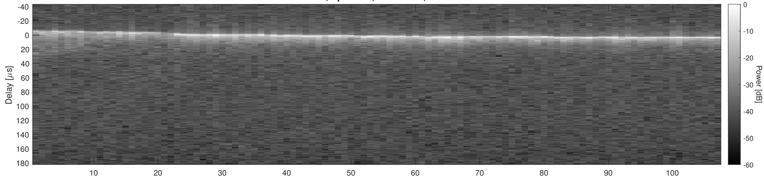
Orbit 3765, Optimized, No Window, Channel 2
