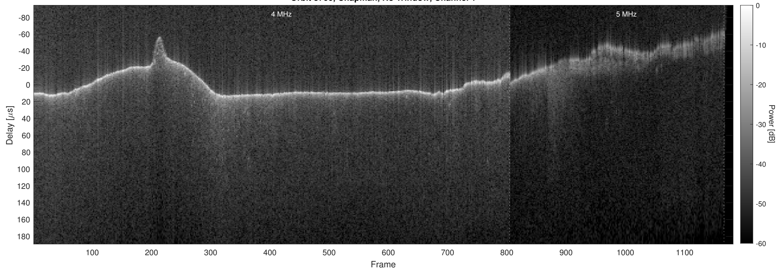
Orbit 3766, Chapman, No Window, Channel 2
