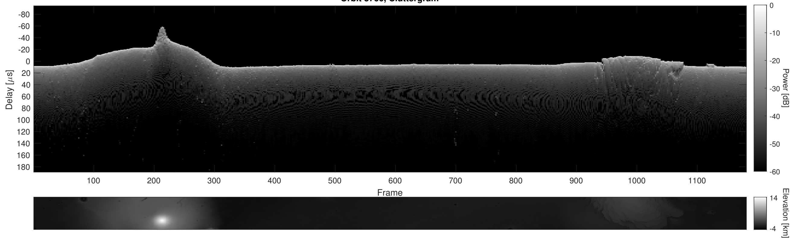
Orbit 3766, Cluttergram
