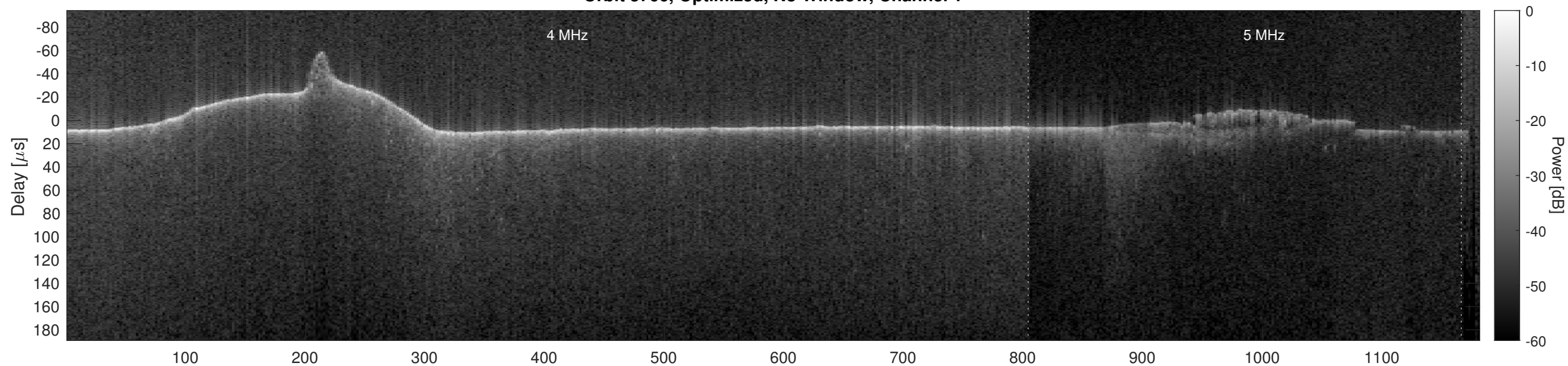
Orbit 3766, Optimized, No Window, Channel 2
