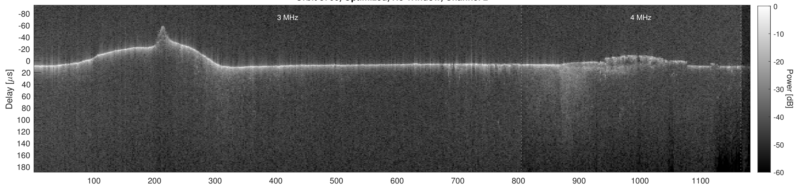
Orbit 3766, Cluttergram
