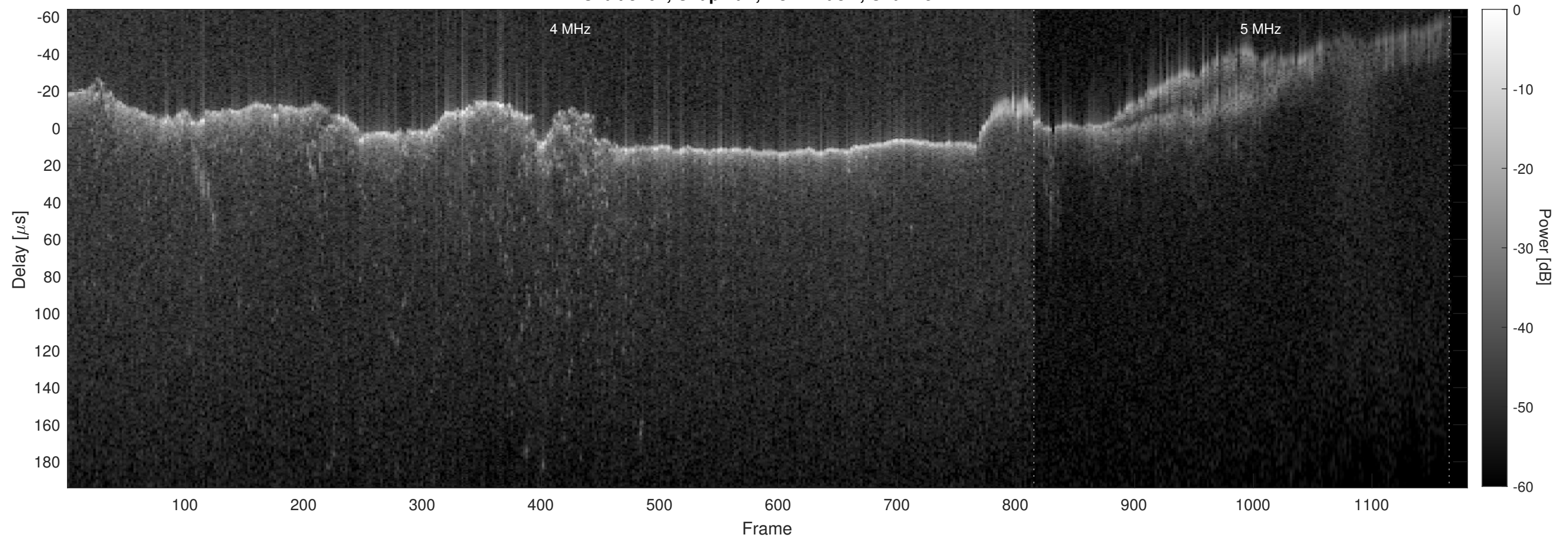
Orbit 3767, Chapman, No Window, Channel 2
