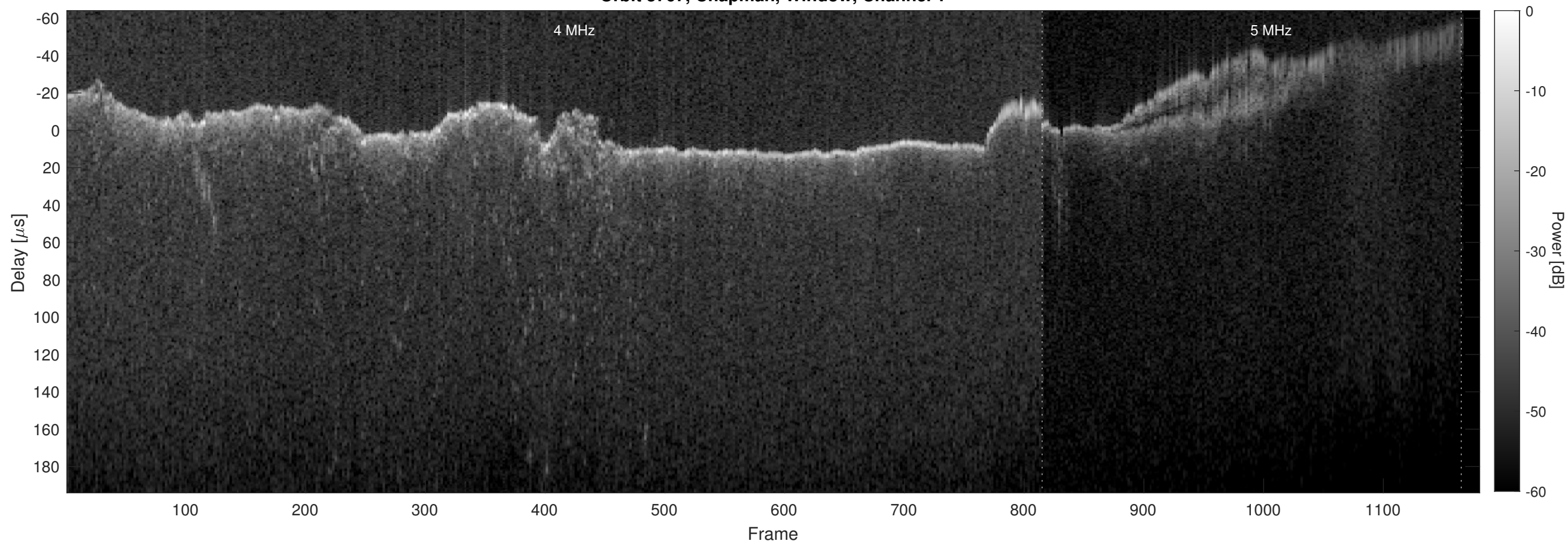
Orbit 3767, Chapman, Window, Channel 2
