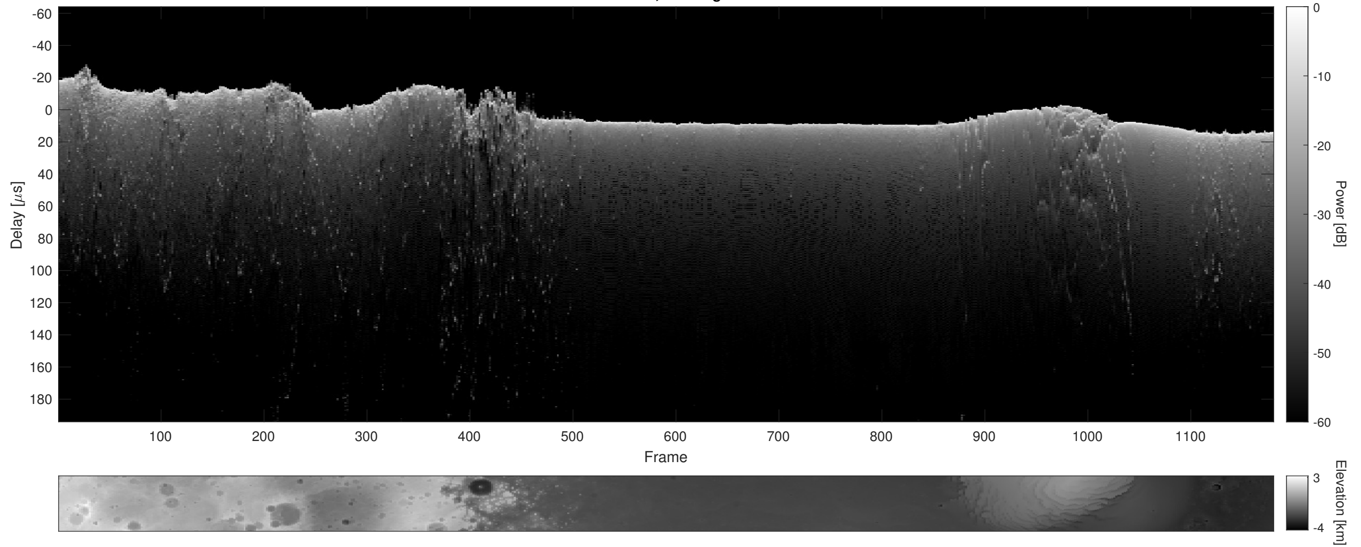
Orbit 3767, Cluttergram
