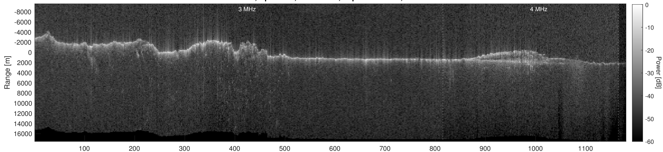
Orbit 3767, Depth-Corrected Cluttergram
