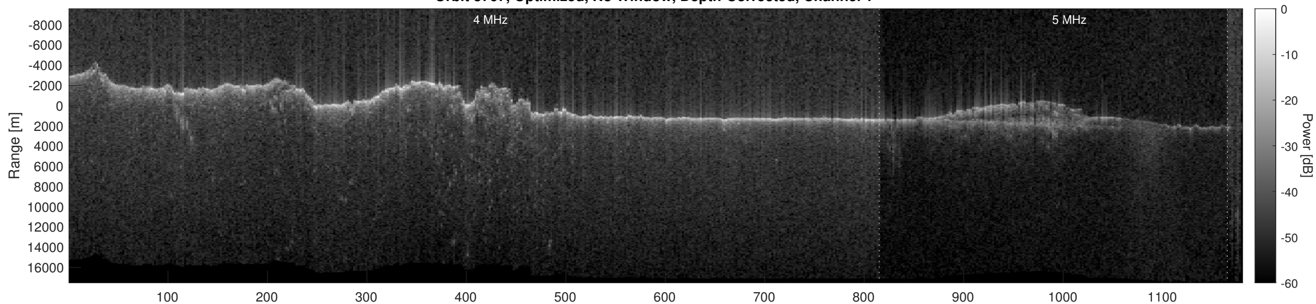
Orbit 3767, Optimized, No Window, Depth-Corrected, Channel 2
