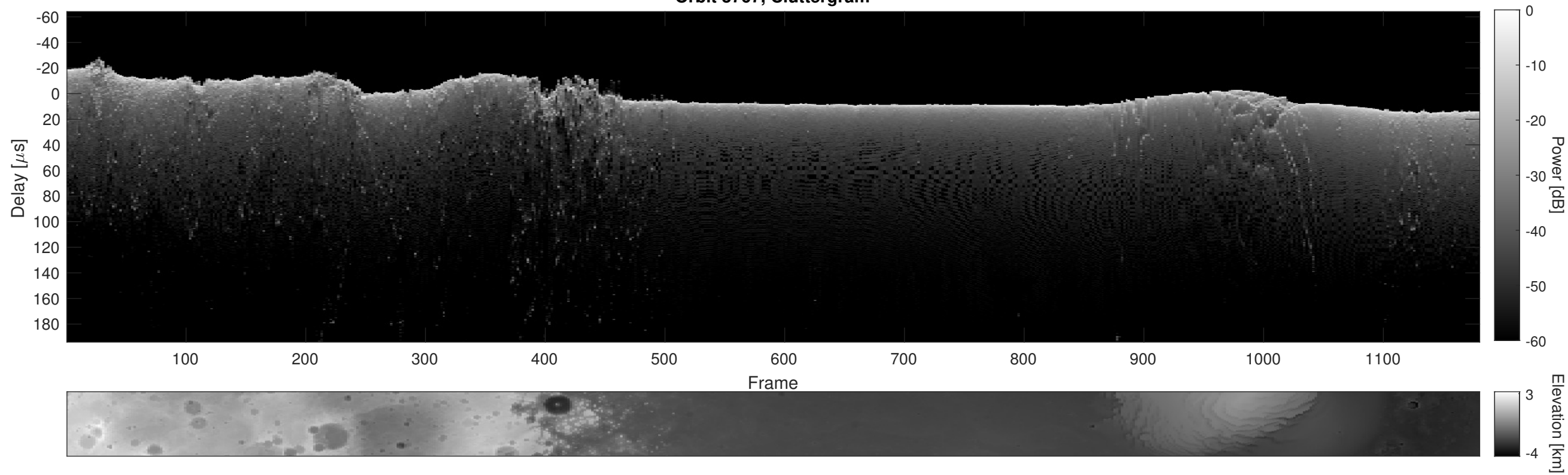
Orbit 3767, Cluttergram
