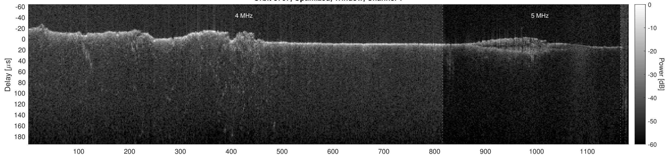
Orbit 3767, Optimized, Window, Channel 2
