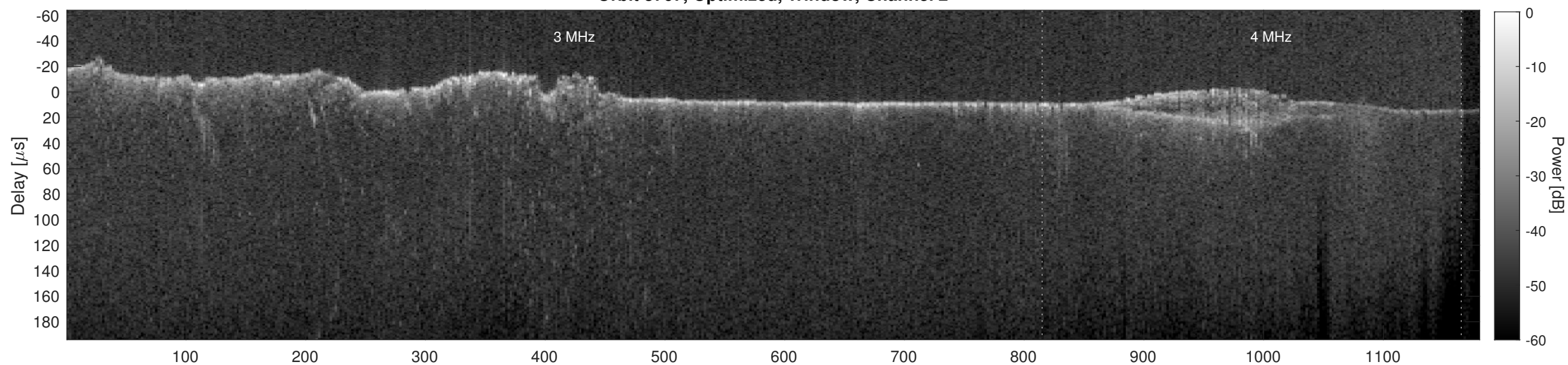
Orbit 3767, Cluttergram
