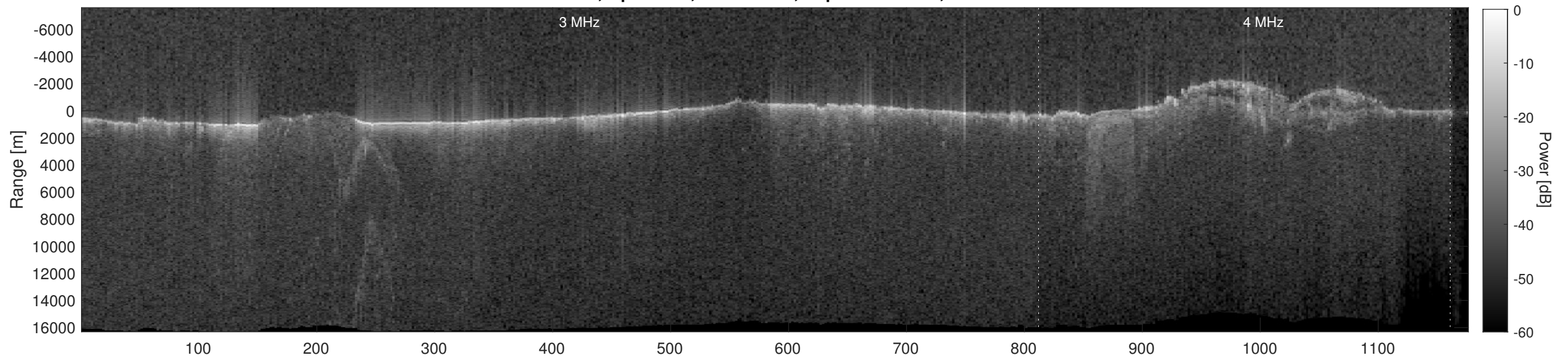
Orbit 3769, Depth-Corrected Cluttergram
