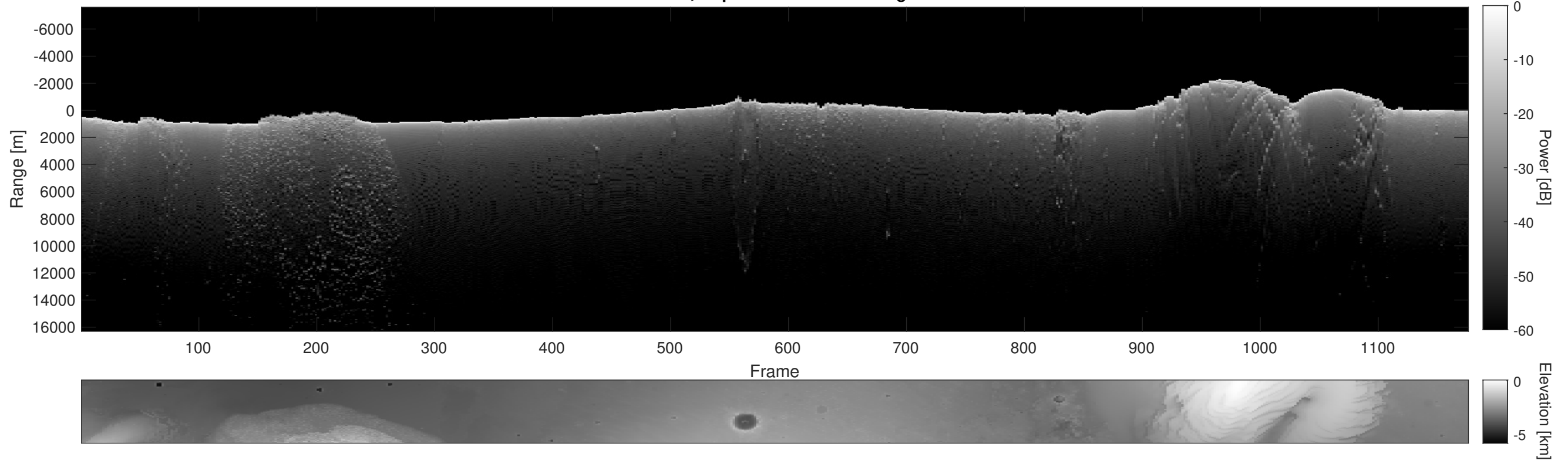
Orbit 3769, Depth-Corrected Cluttergram
