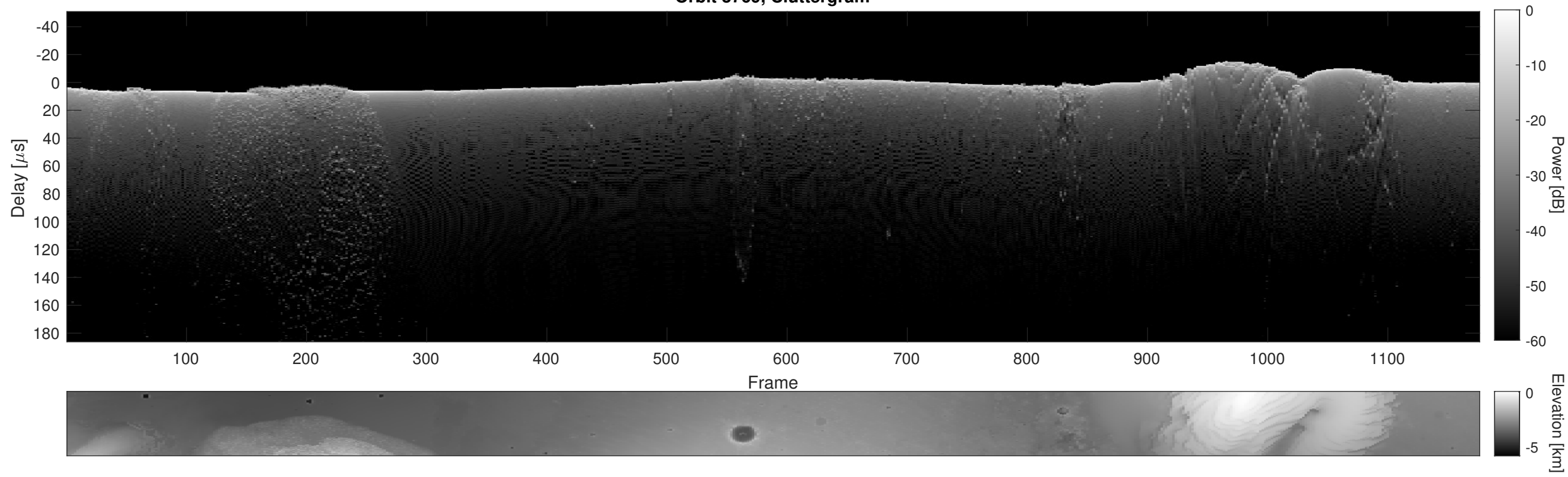
Orbit 3769, Cluttergram
