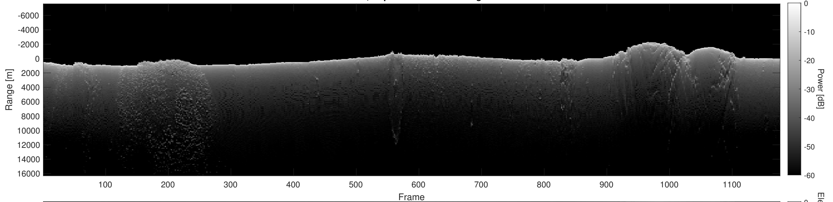
Orbit 3769, Depth-Corrected Cluttergram
