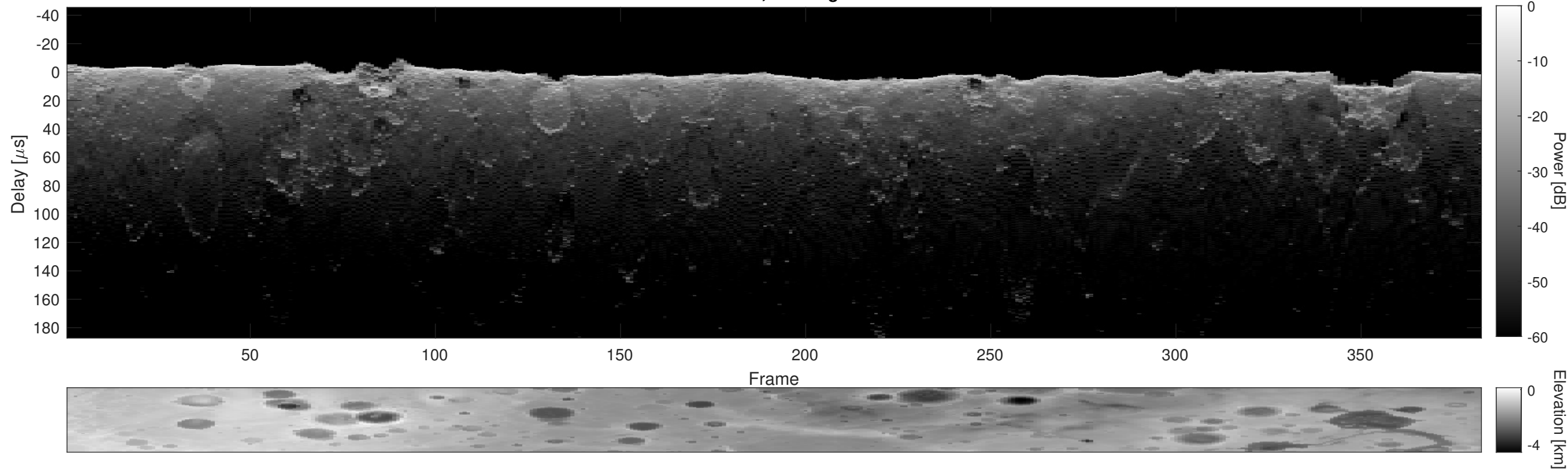
Orbit 3771, Cluttergram
