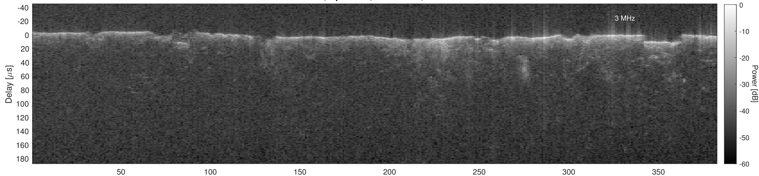
Orbit 3771, Cluttergram
