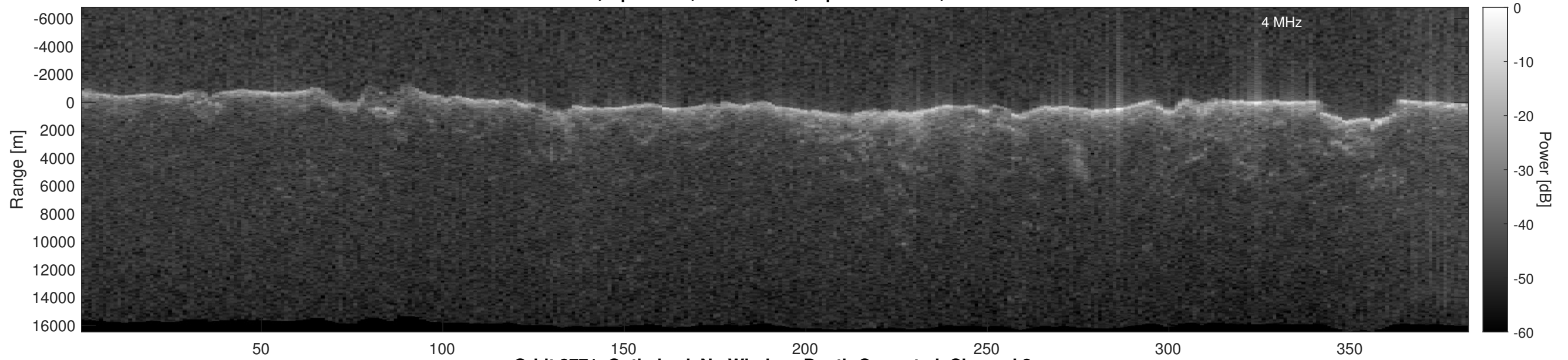
Orbit 3771, Optimized, No Window, Depth-Corrected, Channel 2
