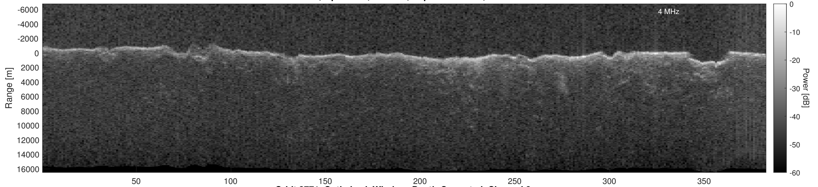
Orbit 3771, Optimized, Window, Depth-Corrected, Channel 2
