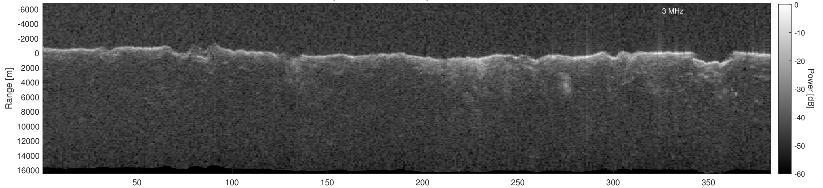
Orbit 3771, Depth-Corrected Cluttergram
