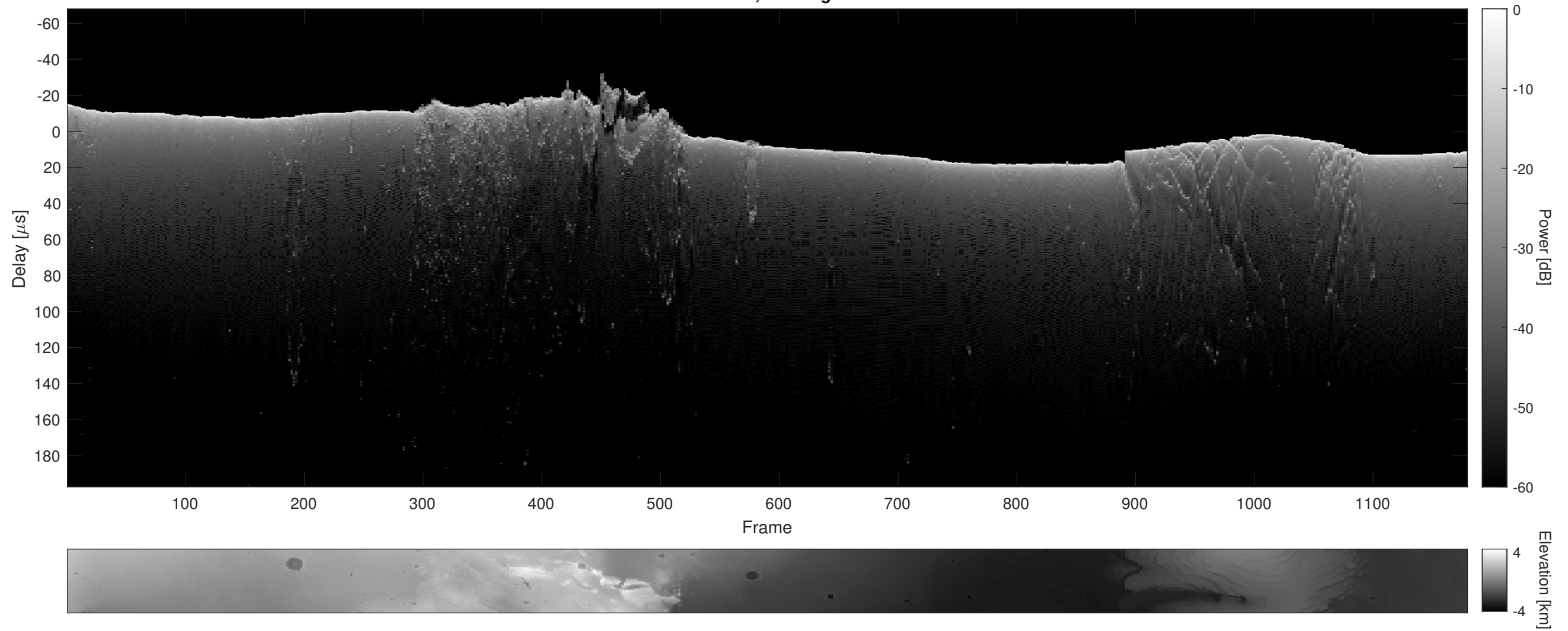
Orbit 3772, Cluttergram
