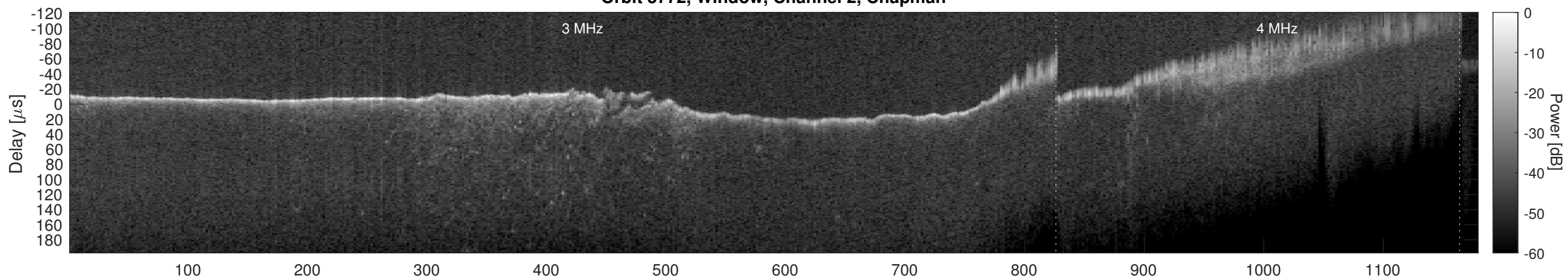
Orbit 3772, Window, Channel 2, Optimized
