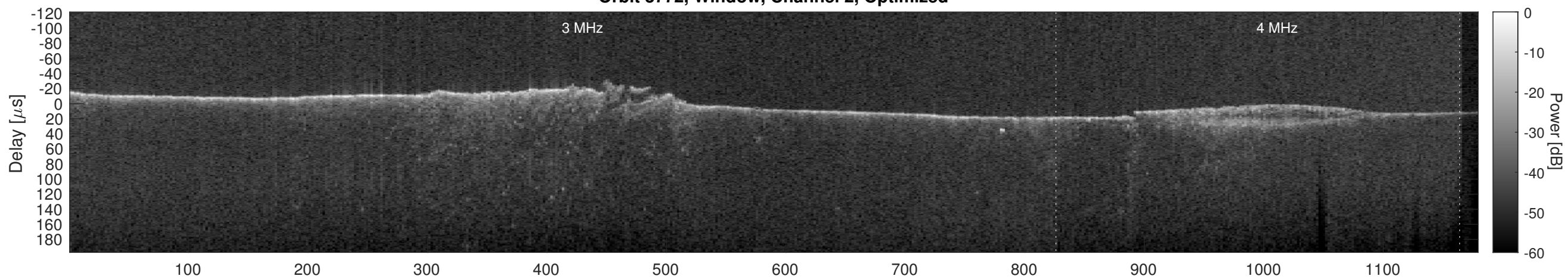
Orbit 3772, Cluttergram
