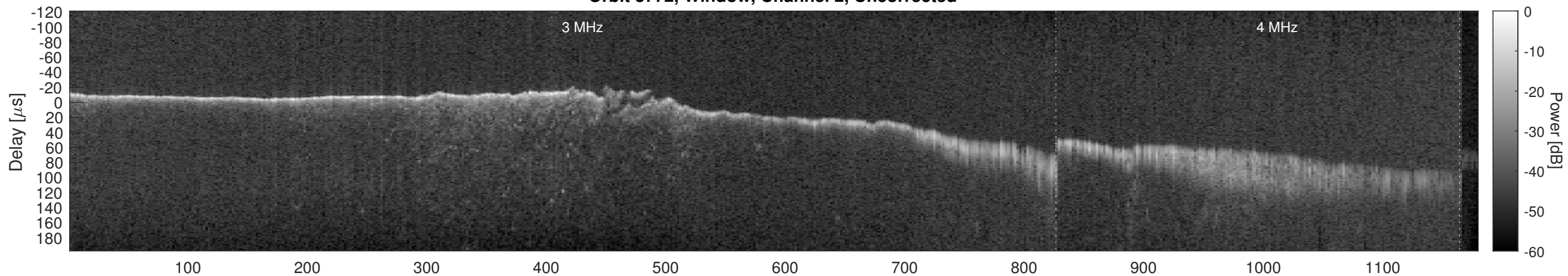
Orbit 3772, Window, Channel 2, Chapman
