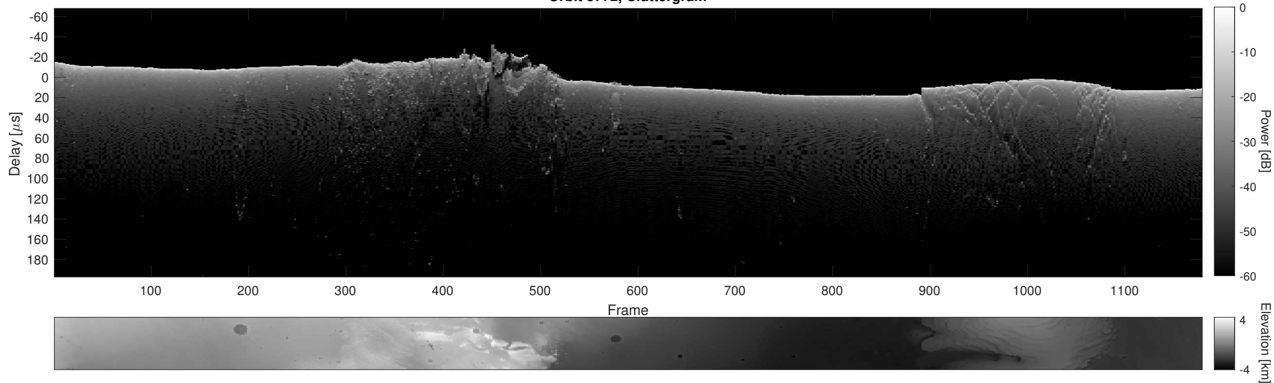
Orbit 3772, Cluttergram
