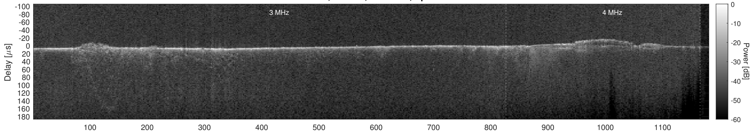
Orbit 3773, Cluttergram
