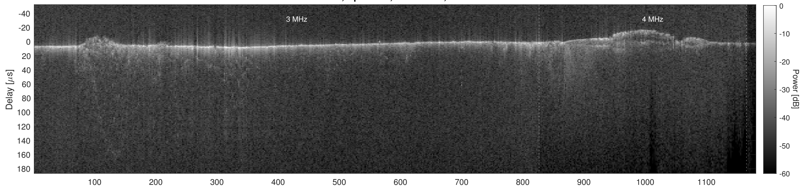
Orbit 3773, Cluttergram
