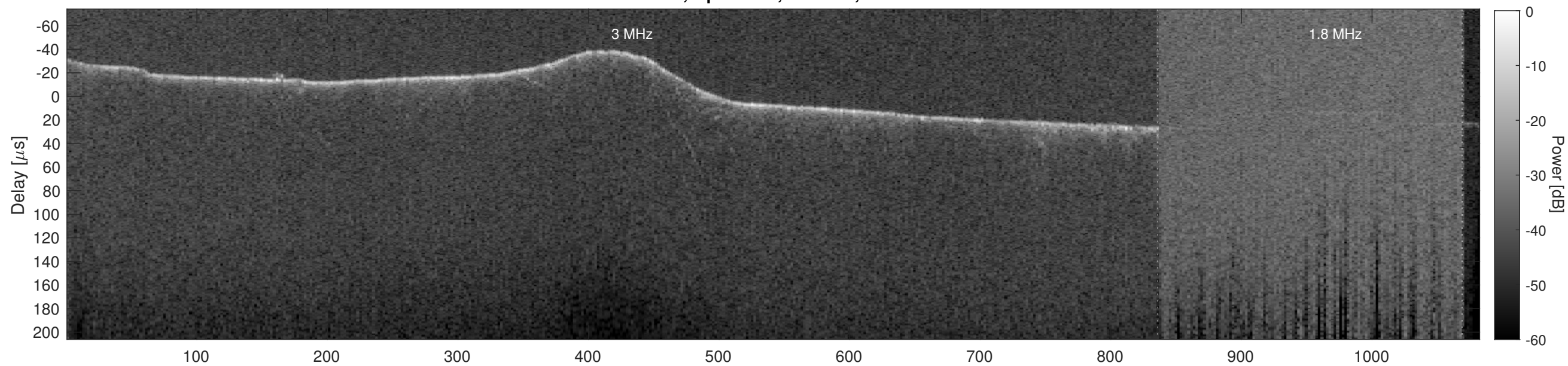
Orbit 3776, Cluttergram
