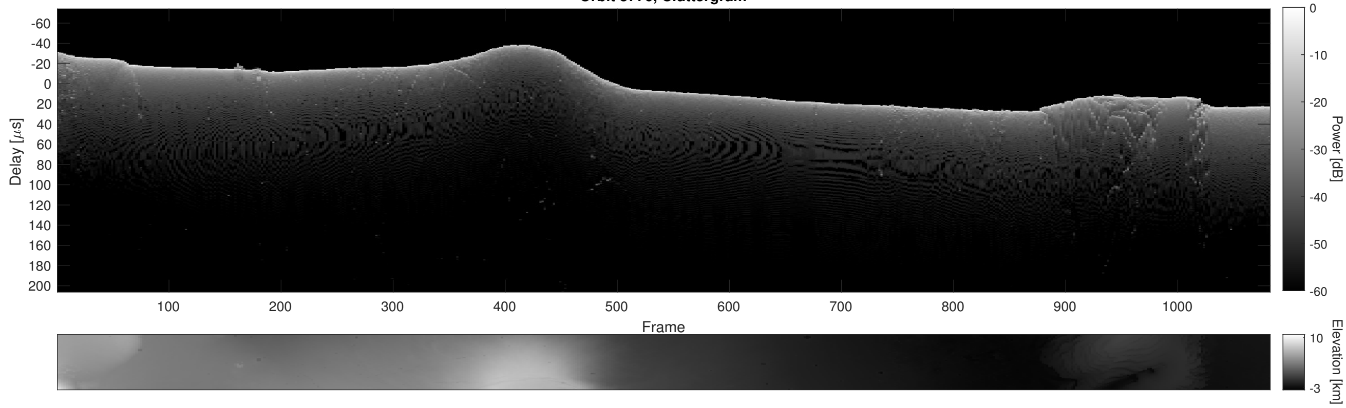
Orbit 3776, Cluttergram
