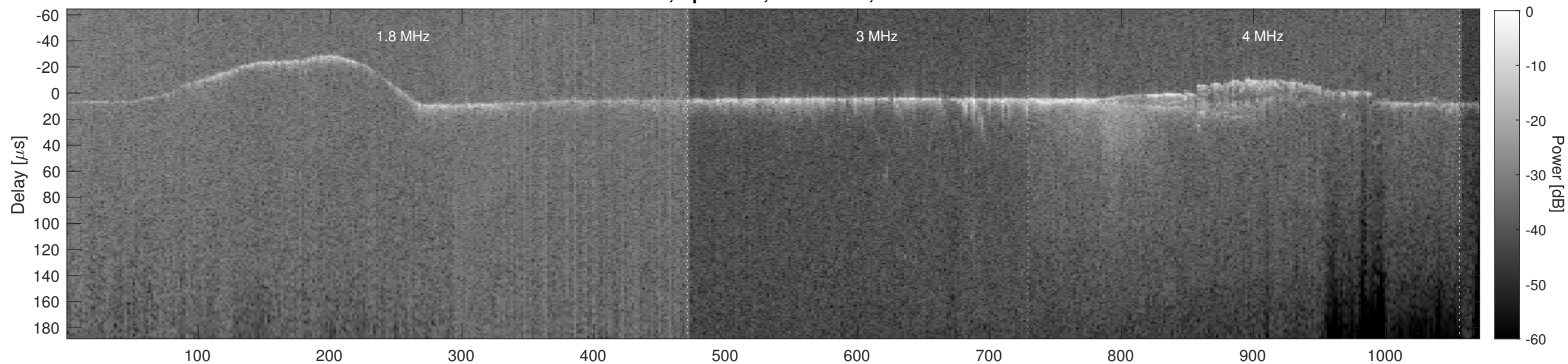
Orbit 3777, Cluttergram
