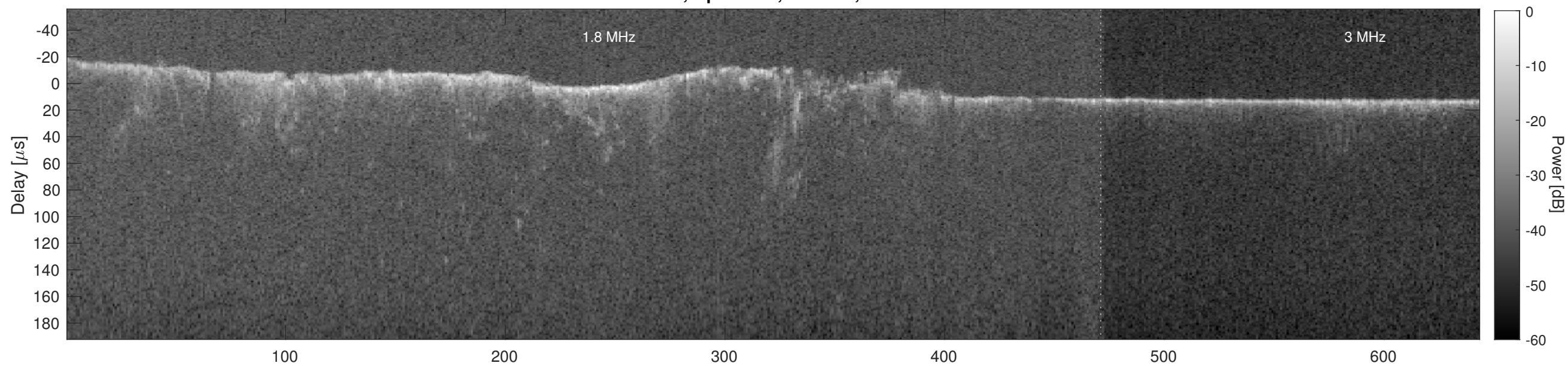
Orbit 3778, Cluttergram
