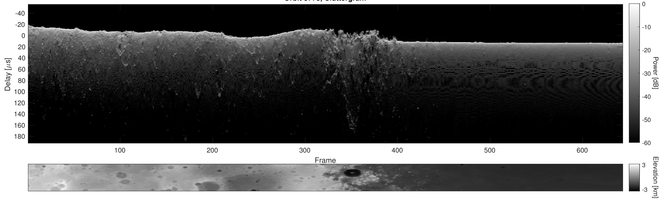
Orbit 3778, Cluttergram
