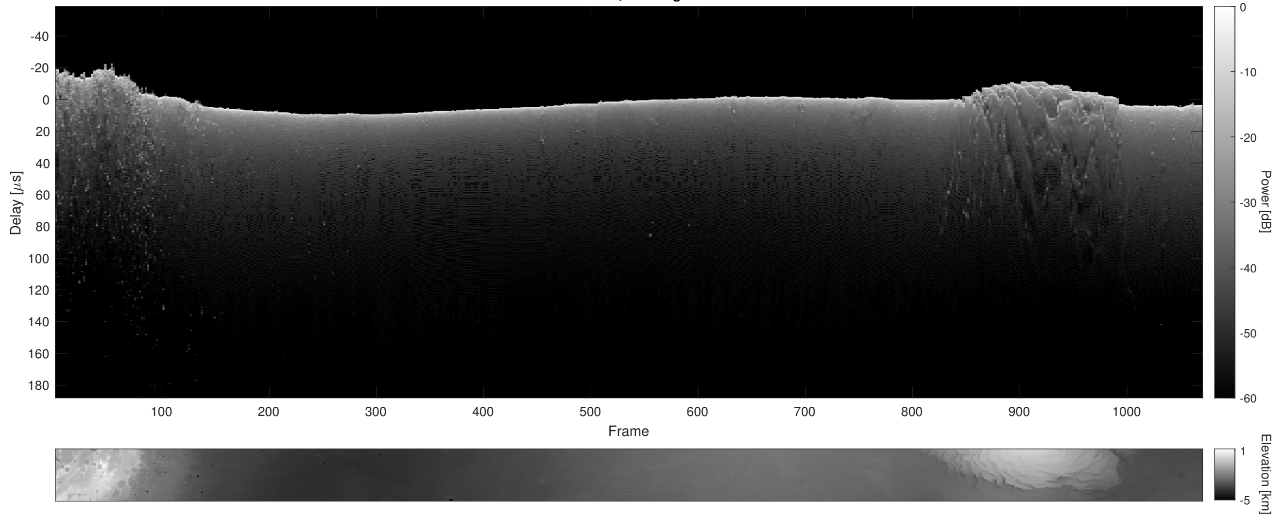
Orbit 3781, Cluttergram
