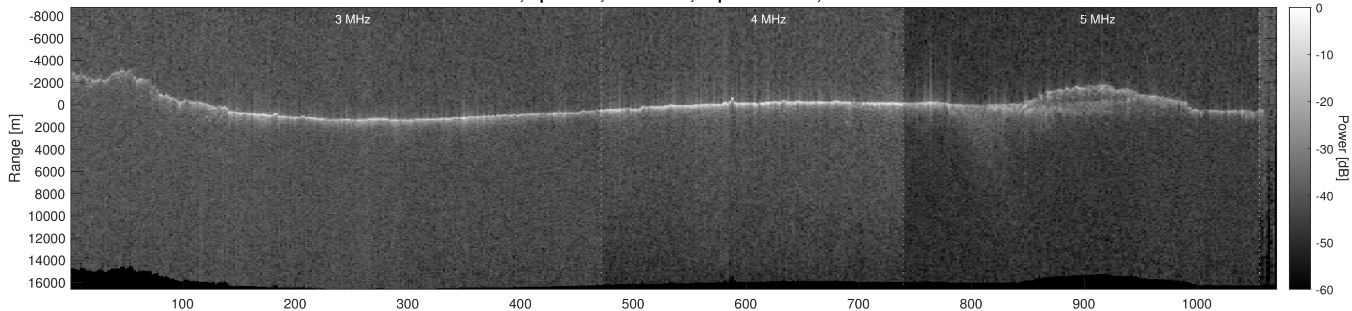
Orbit 3781, Optimized, No Window, Depth-Corrected, Channel 2
