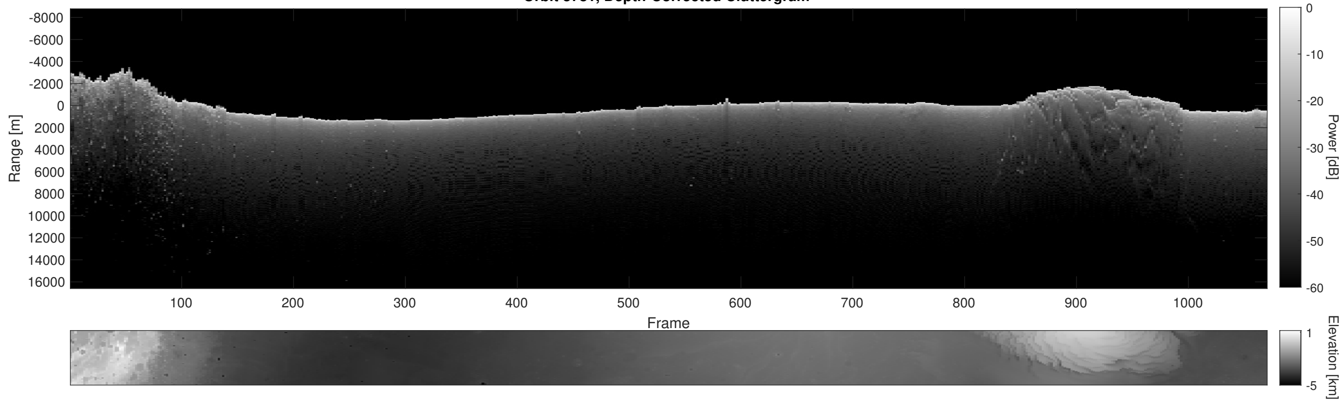
Orbit 3781, Depth-Corrected Cluttergram
