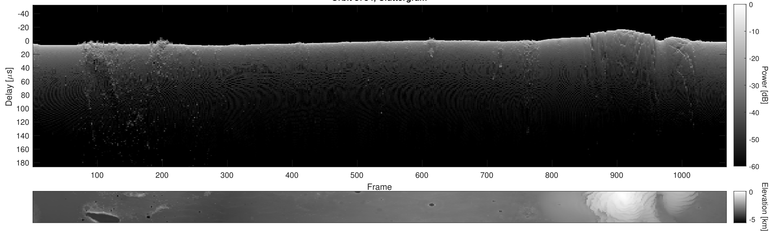
Orbit 3784, Cluttergram
