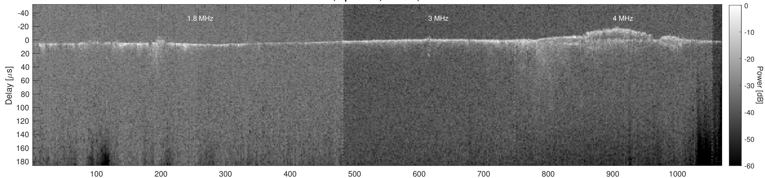
Orbit 3784, Cluttergram
