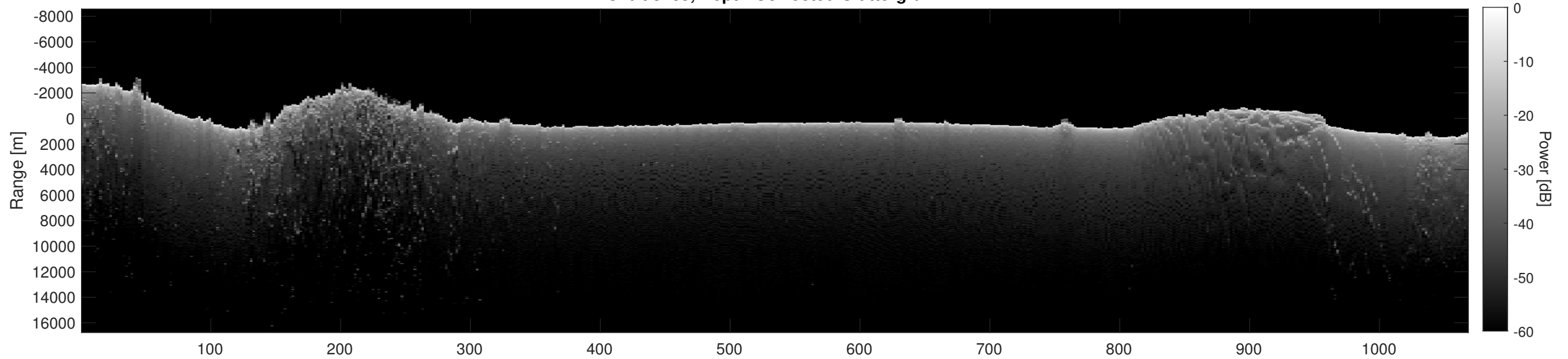
Orbit 3785, Depth-Corrected Cluttergram
