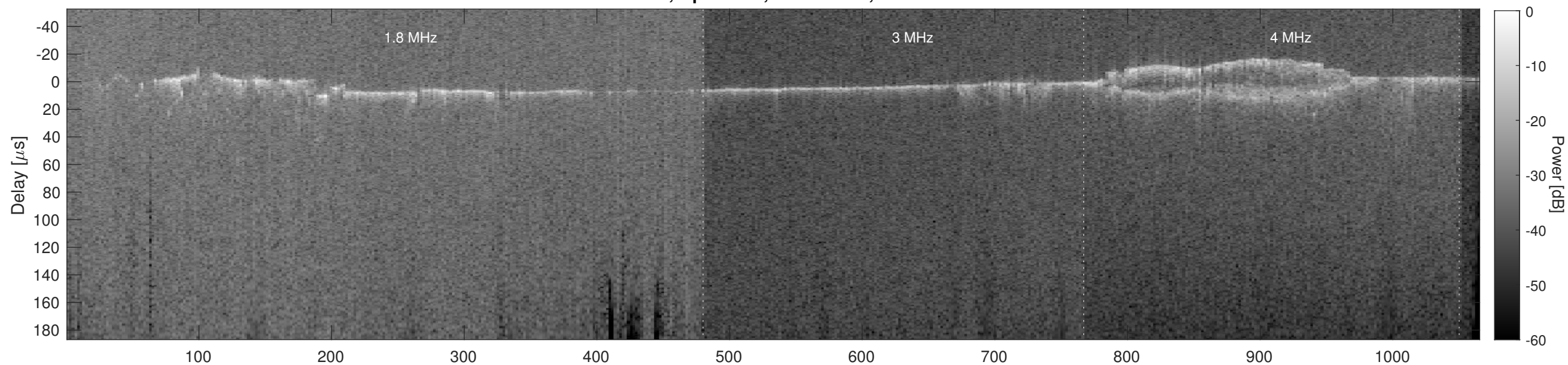
Orbit 3786, Cluttergram
