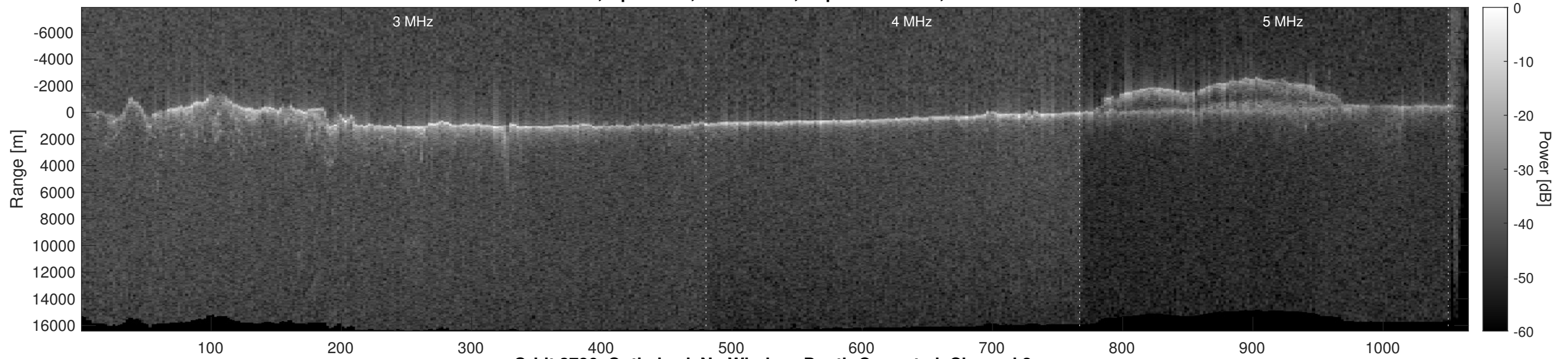
Orbit 3786, Optimized, No Window, Depth-Corrected, Channel 2
