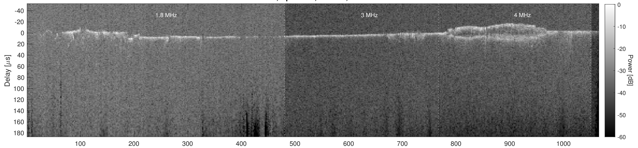
Orbit 3786, Cluttergram
