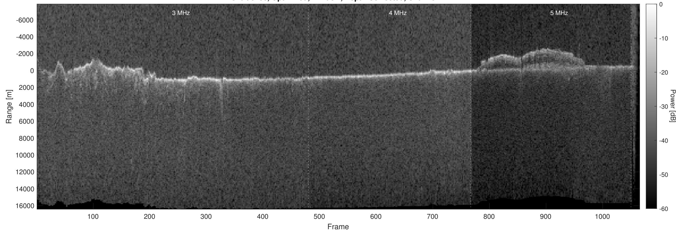
Orbit 3786, Optimized, Window, Depth-Corrected, Channel 2
