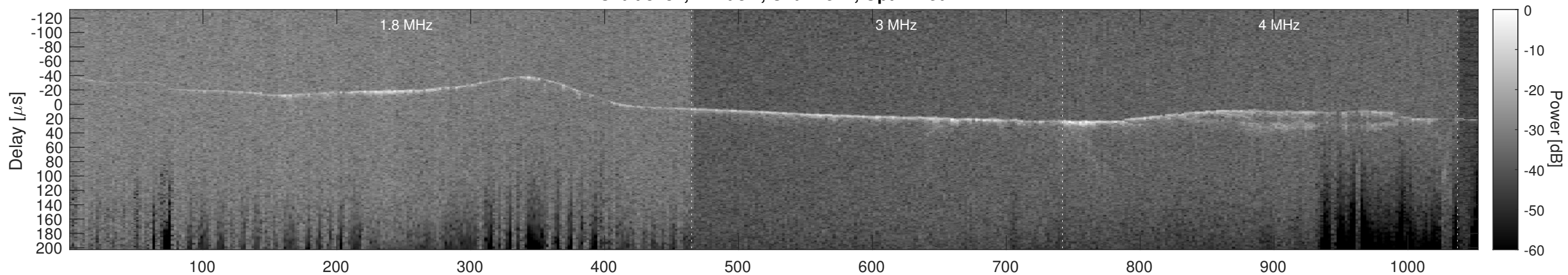
Orbit 3787, Cluttergram
