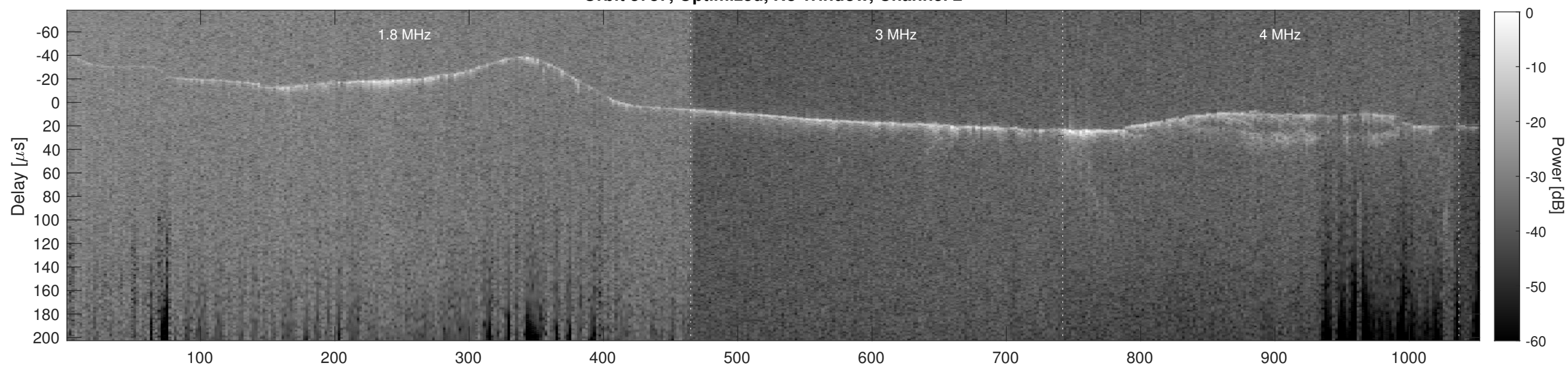
Orbit 3787, Cluttergram
