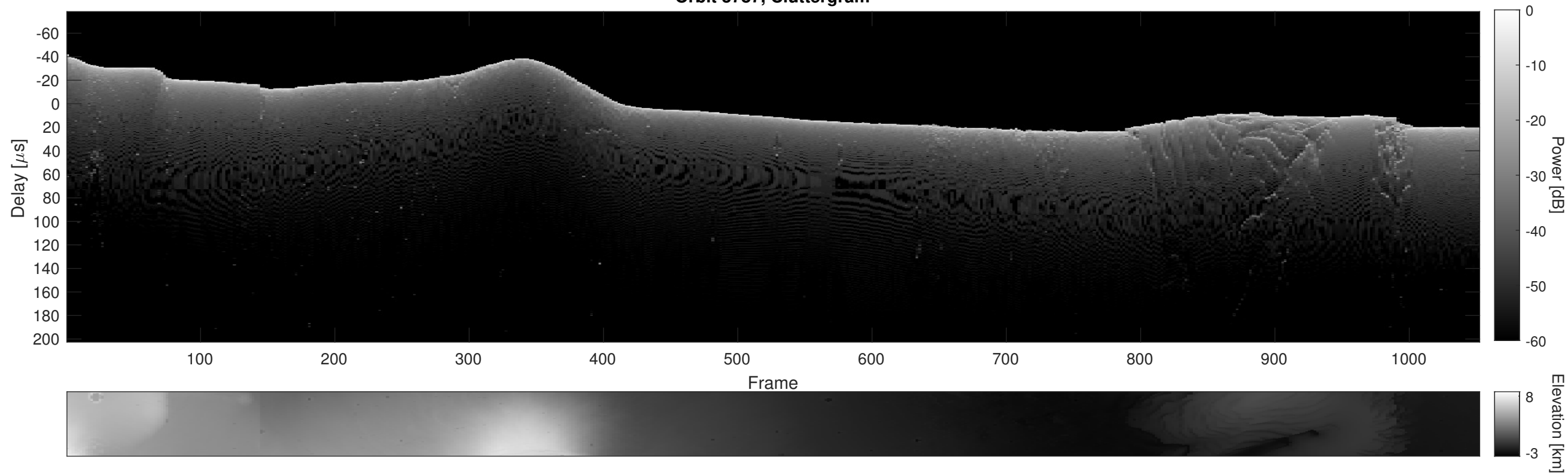
Orbit 3787, Cluttergram
