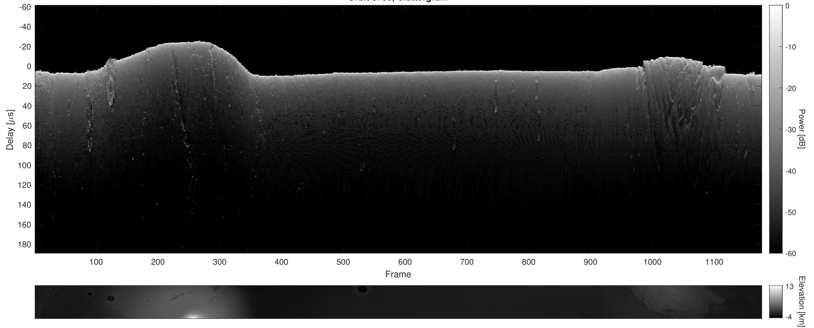
Orbit 3788, Cluttergram
