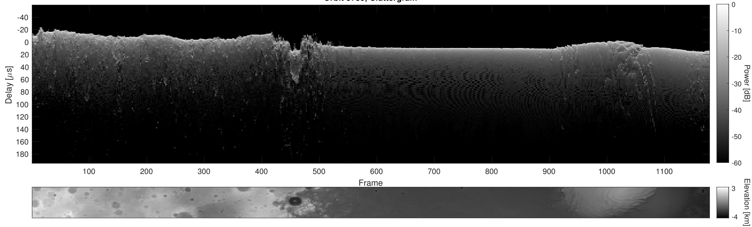
Orbit 3789, Cluttergram
