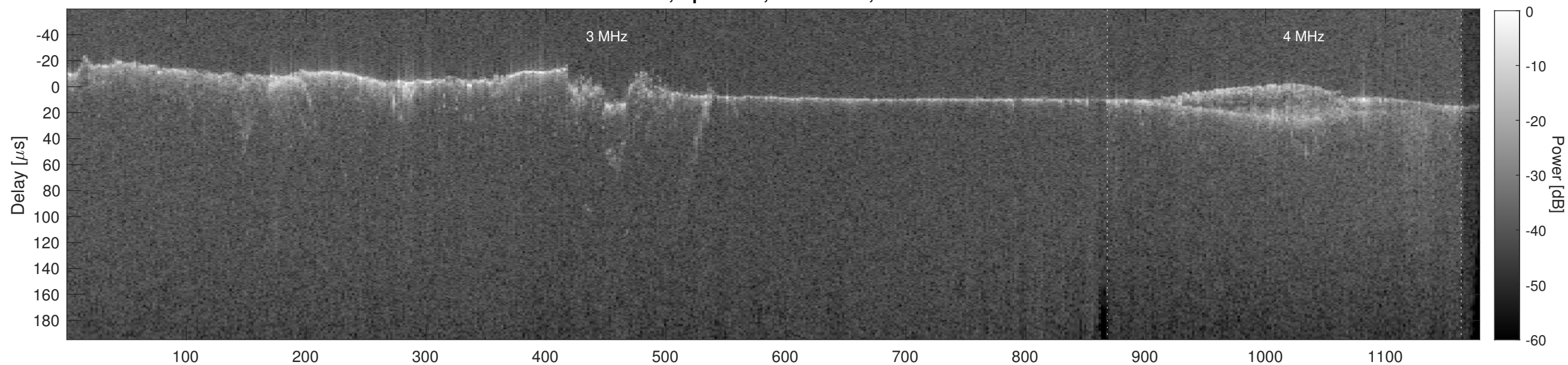
Orbit 3789, Cluttergram
