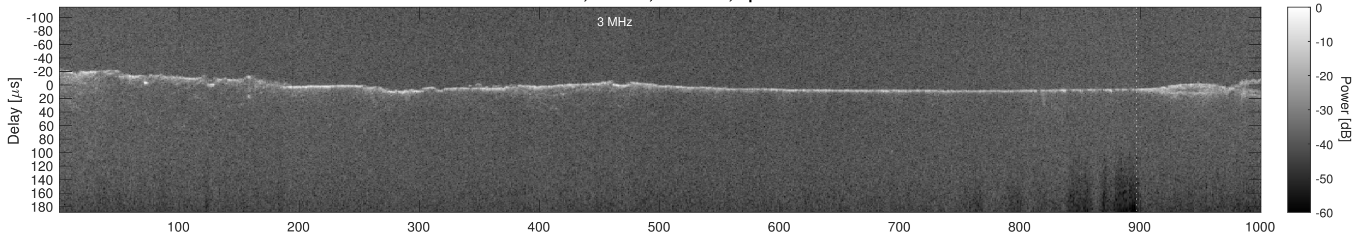
Orbit 3790, Cluttergram
