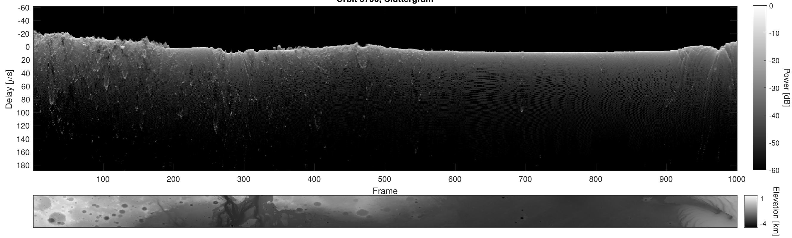
Orbit 3790, Cluttergram
