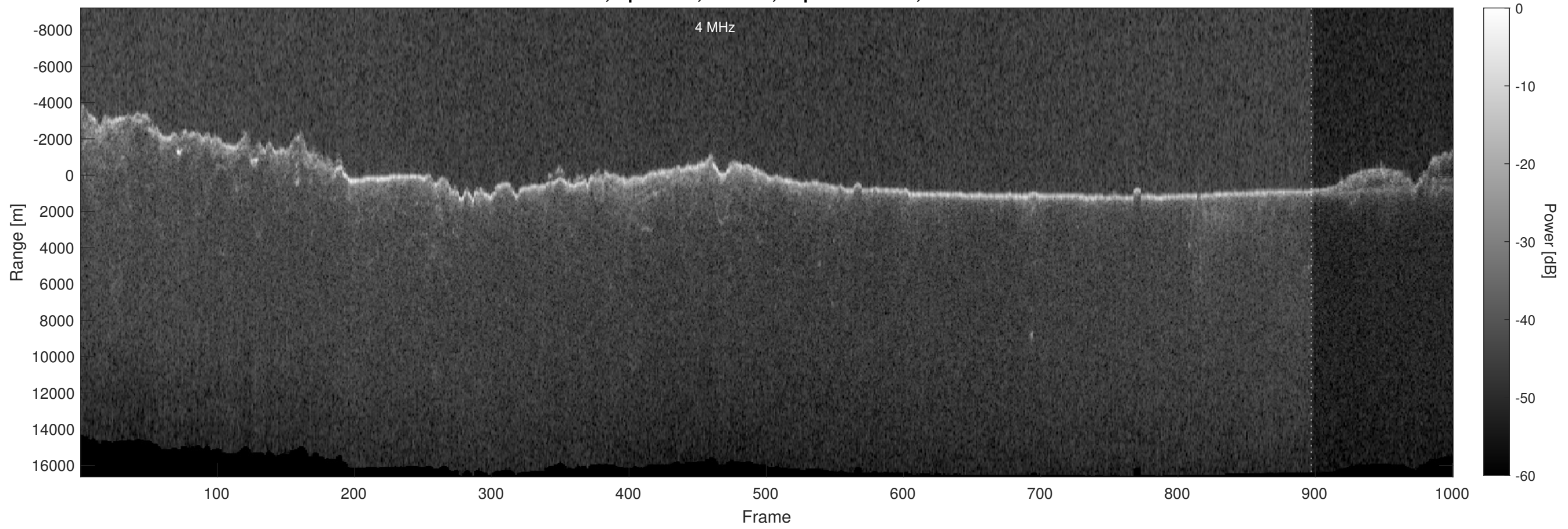
Orbit 3790, Optimized, Window, Depth-Corrected, Channel 2
