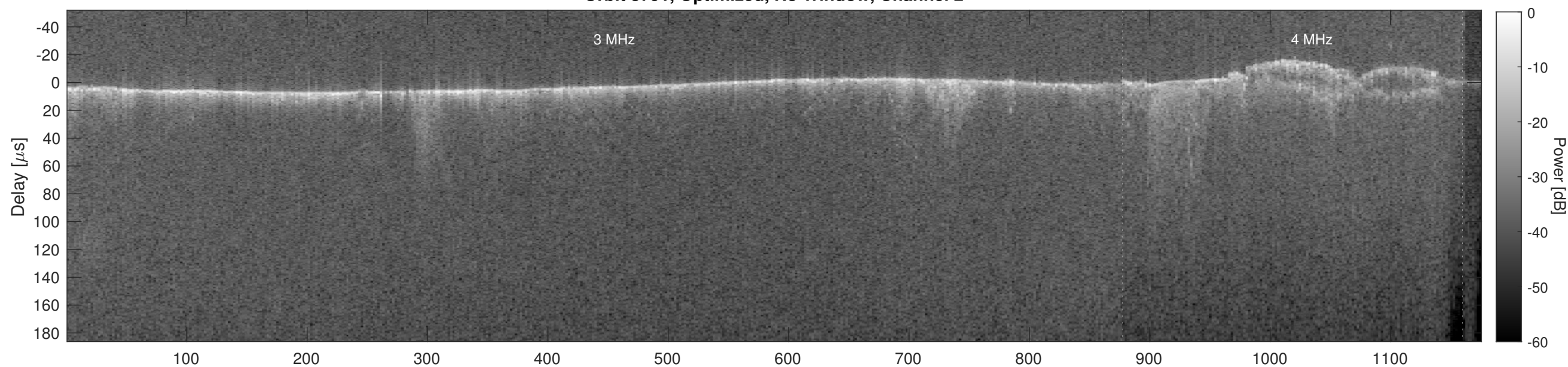
Orbit 3791, Cluttergram
