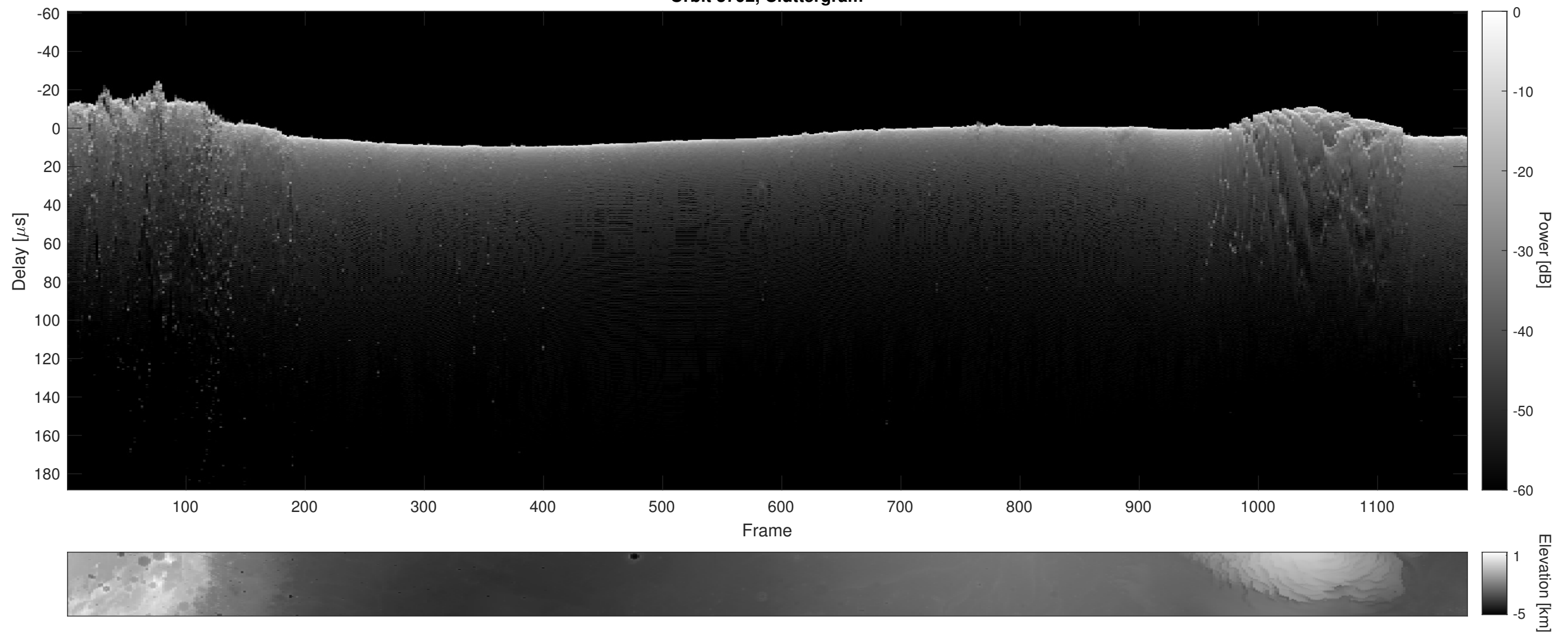
Orbit 3792, Cluttergram
