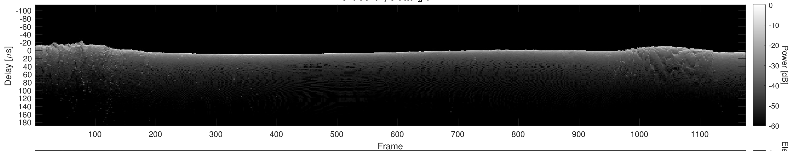
Orbit 3792, Cluttergram
