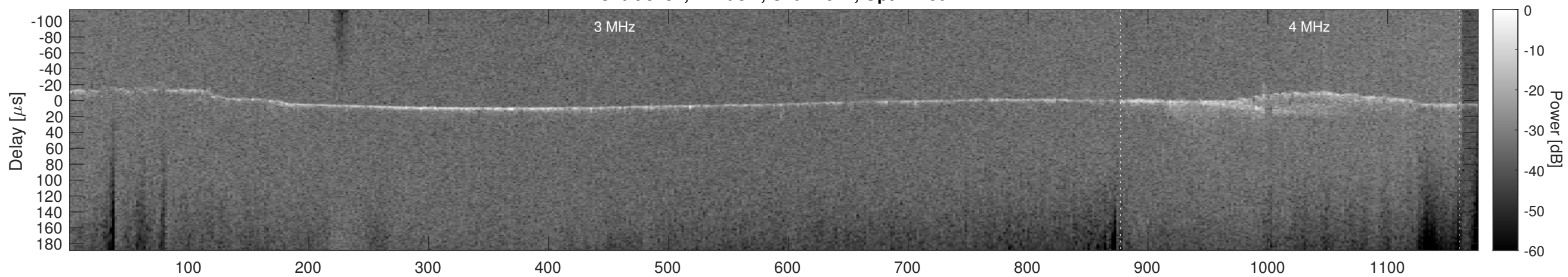
Orbit 3792, Cluttergram
