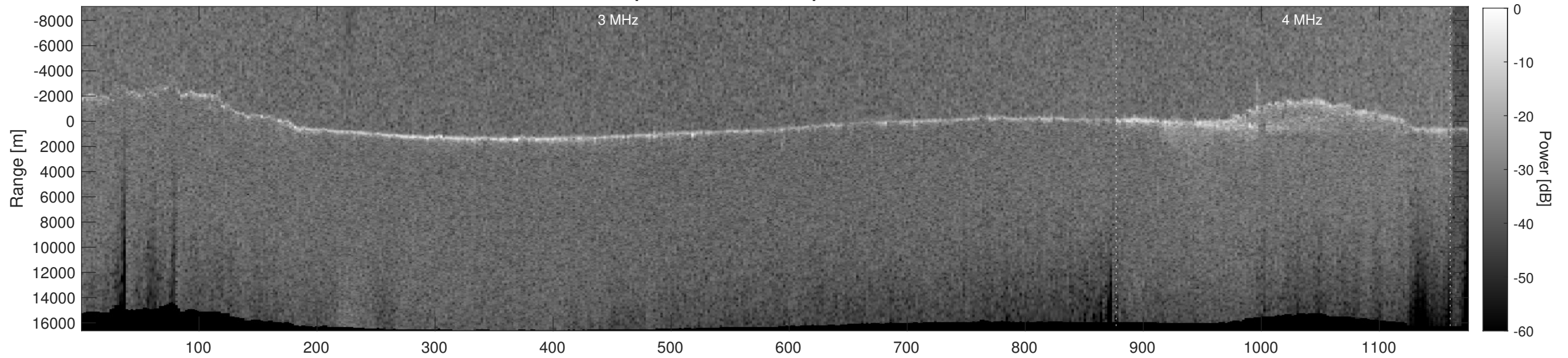
Orbit 3792, Depth-Corrected Cluttergram
