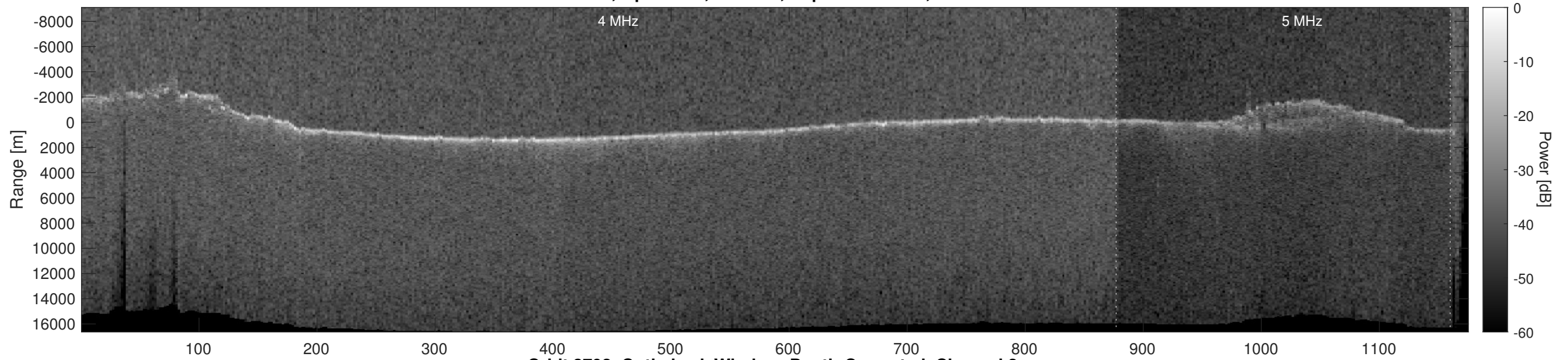
Orbit 3792, Optimized, Window, Depth-Corrected, Channel 2
