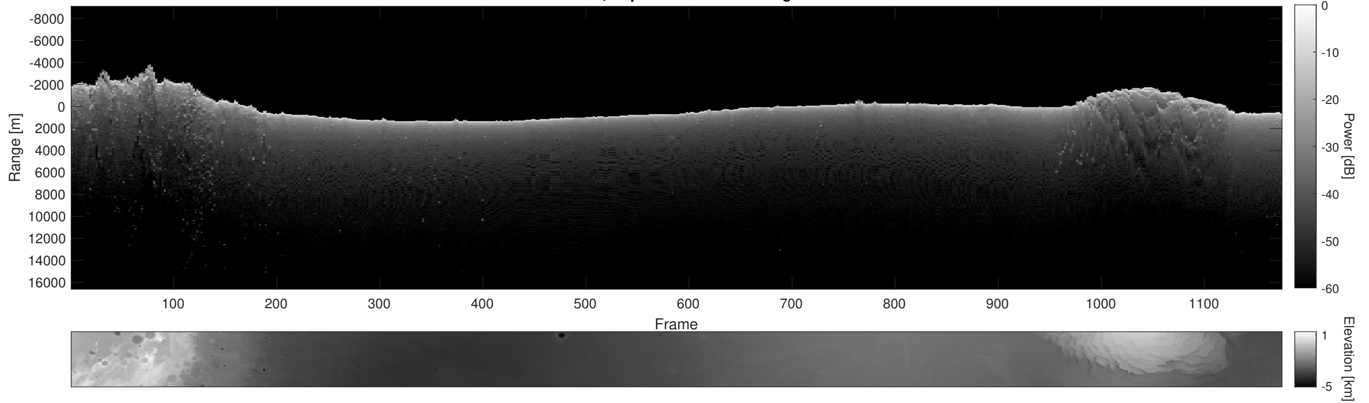
Orbit 3792, Depth-Corrected Cluttergram
