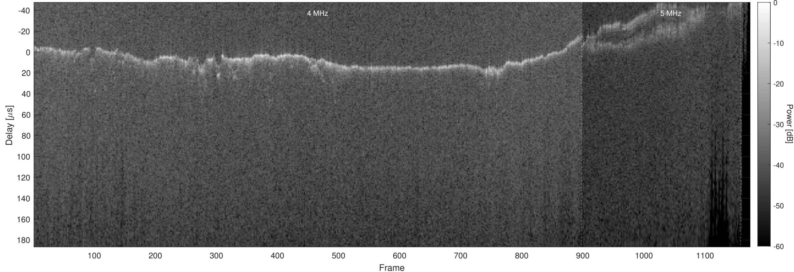
Orbit 3793, Chapman, No Window, Channel 2
