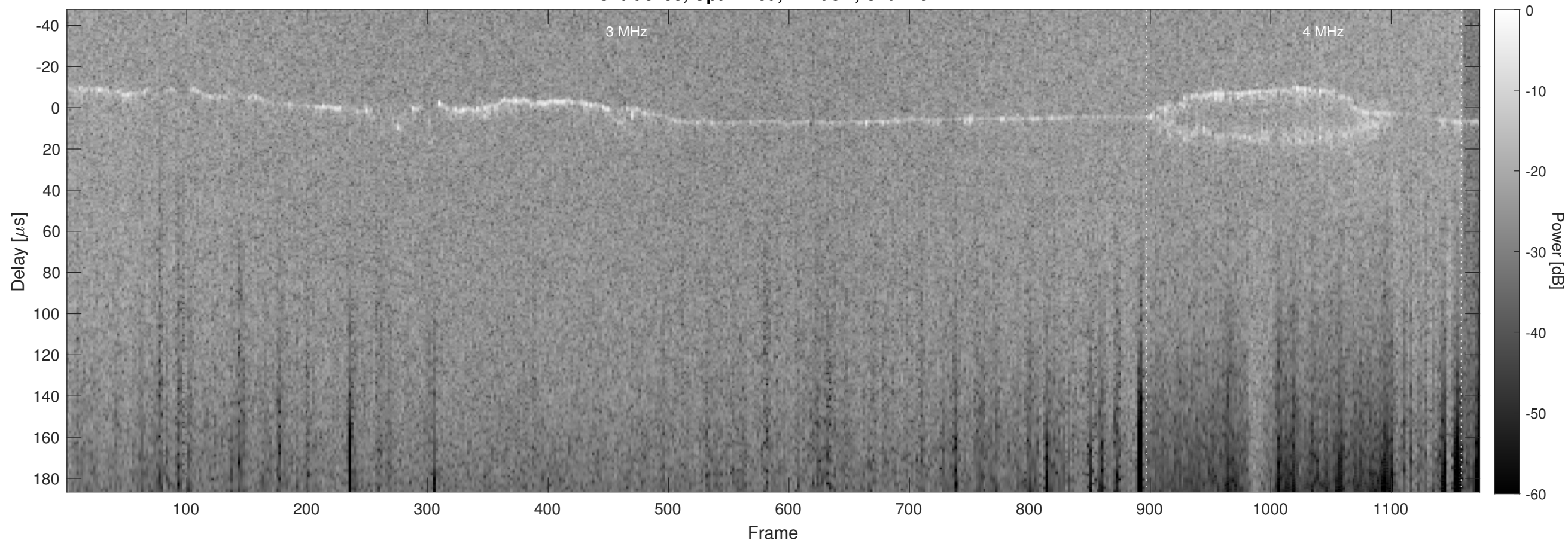
Orbit 3793, Optimized, Window, Channel 2
