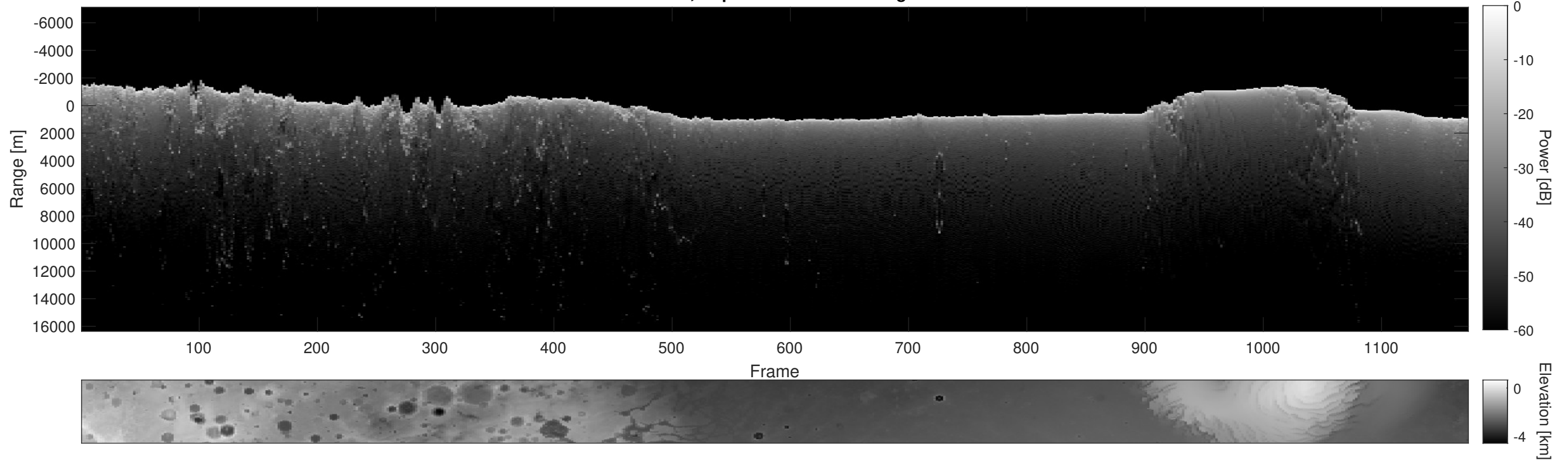
Orbit 3793, Depth-Corrected Cluttergram
