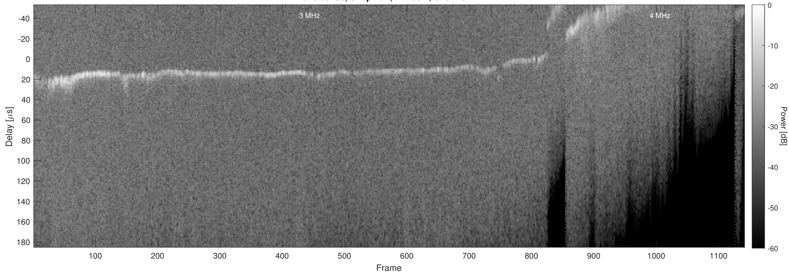
Orbit 3795, Chapman, Window, Channel 2
